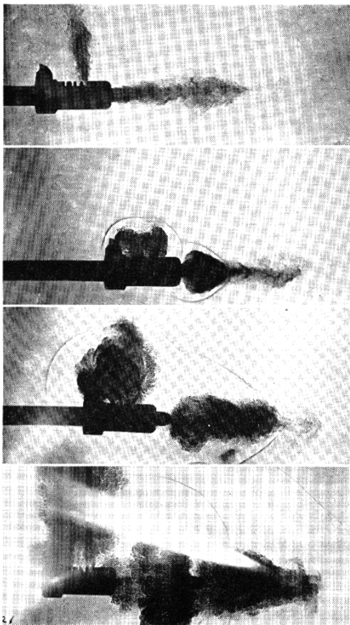
Series of spark photographs made by the late Capt. Philip Quayle for Col. R. M. Cutts and published with the permission of the latter. These show how gas escapes between the expanded neck of the cartridge case and the bullet, before the latter starts forward. If the necks did not let go of those bullets first, how did that gas get out ahead of them?
