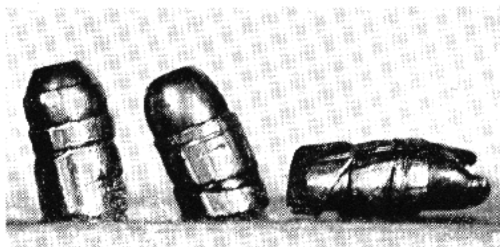
Hollow base bullets in which the cavity was carried too deep. When fired, the bullet slugged badly or the base blew out and the sides collapsed.
