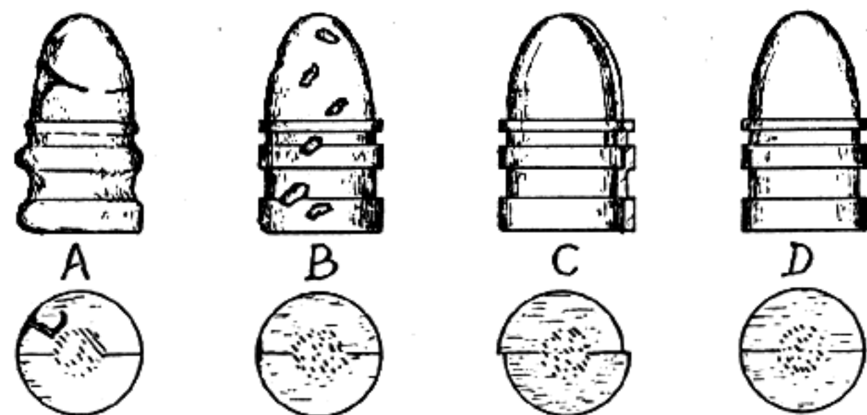
A—Bullet not filled out. Metal or mould too cold. B. Effect of grease or oil in mould. C. Two halves of bullet do not match. Mould has excessive "shuck". D. Perfect Bullet.
