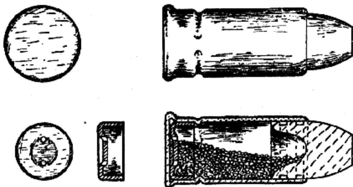
An early center fire cartridge—made with an internal primer.
