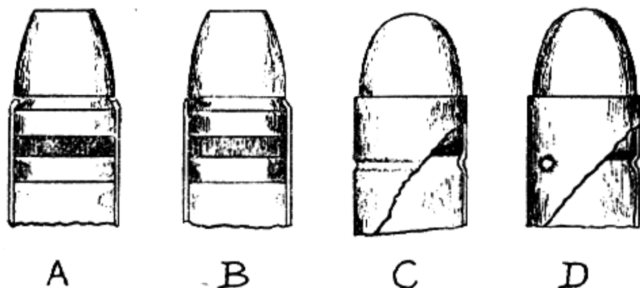
Bullet crimps and cartridge cannellures. A —Bullet crimped into mouth of case. B —Imperfect crimp, deeper on right side than on left. C —45 Auto case, with square shoulder at mouth and case cannellured to prevent bullet from seating too deep. D —Same as C except case is indented instead of cannellured.
