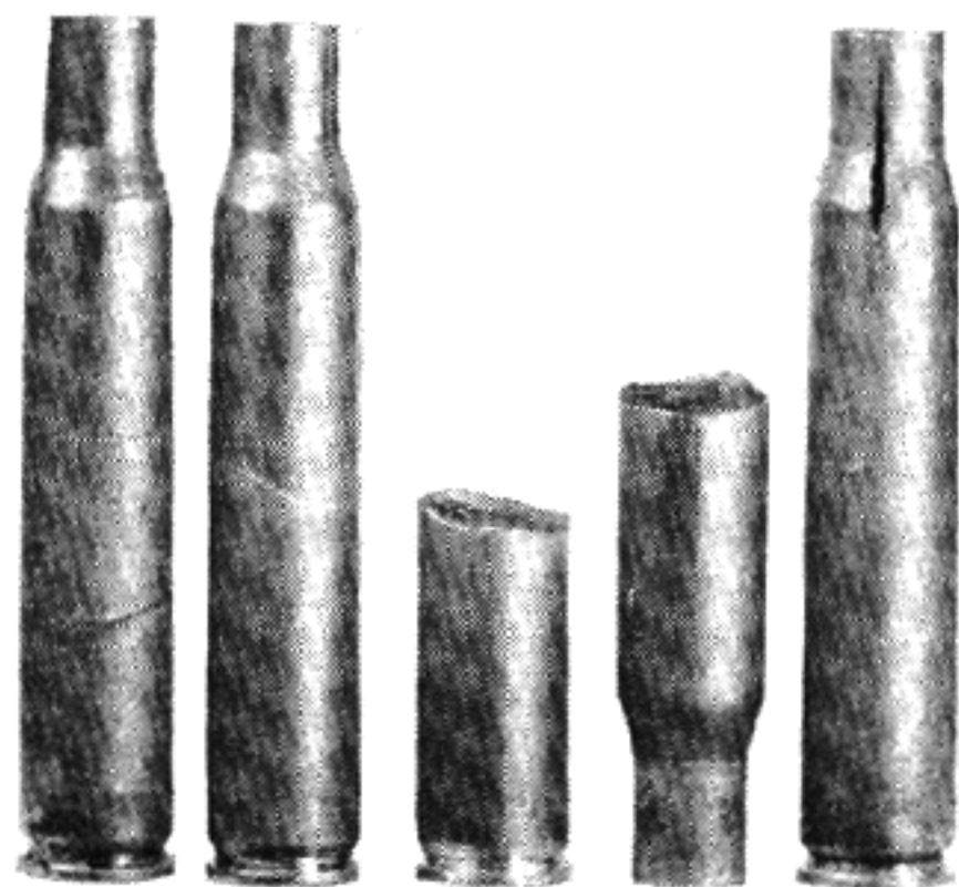
Split and ruptured cartridge cases.
