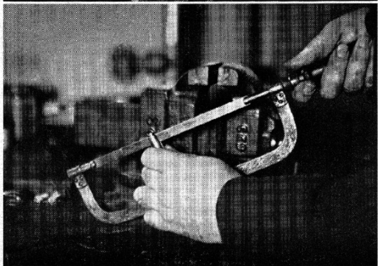
Method of sectioning fired cartridge case to prepare it for etching.
