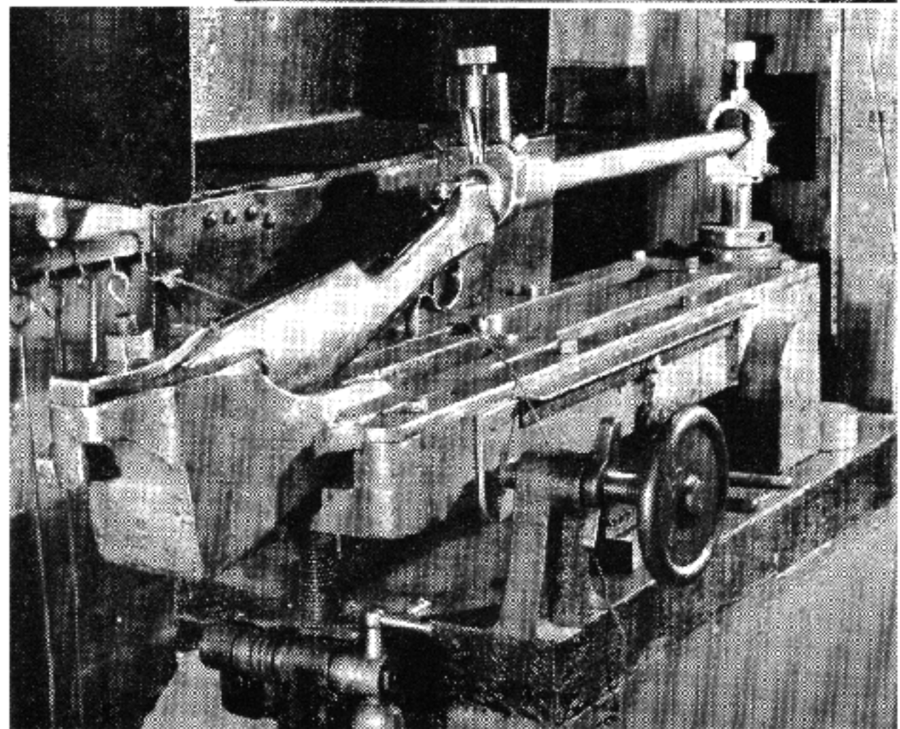
Apparatus for the taking of pressures and velocities. Upper view shows chronograph room of the Hercules Powder Company's ballistic station at Kenil, N. J. Chronograph is set for the taking of time interval as soon as the shot is fired. Lower view shows firing point with rifle set in the rest for taking of both velocity and pressure. Rifle is special pressure gun with yoke mounted over the chamber for the taking of pressures by radial system.
