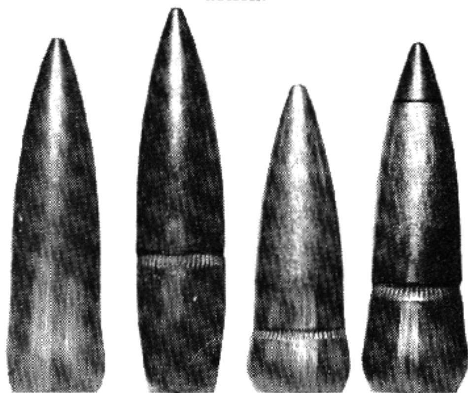
Showing upsettage of bases of flat base bullets in comparison with a boat-tail bullet which does not upset when fired. Upsettage depends upon the structure of the bullet, its hardness, the force applied behind it and the suddenness with which the force is applied.
