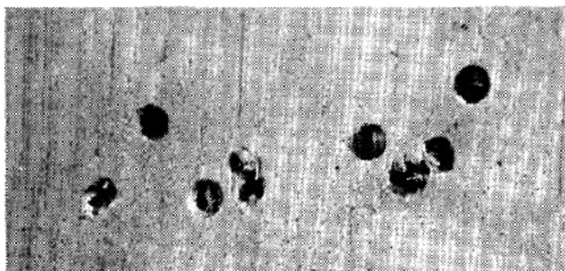
A crude test of primer performance. Two "groups" made by firing the primers from the inside of the cup. Note the deep penetration of the left hand group. This indicates violence but the primers in the right hand group were, by far, the best ignitors of the two.
