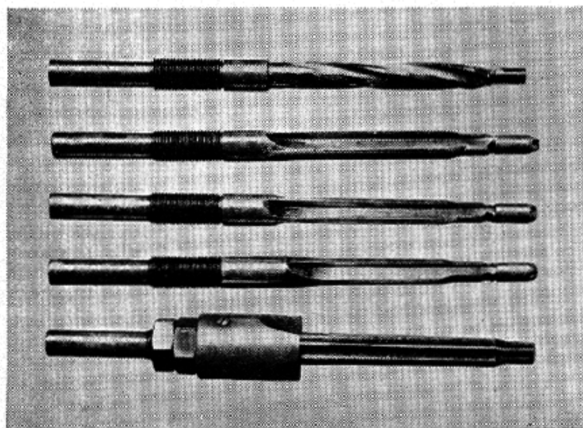
A Set of Machine Gun Chambering Reamers.
